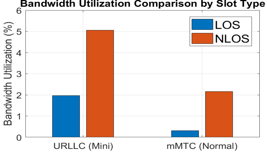
Figure 9: Bandwidth Utilization Comparison by Slot Type
