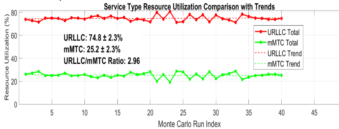
Figure 13: Service Type Resource Utilization Comparison with Trends
