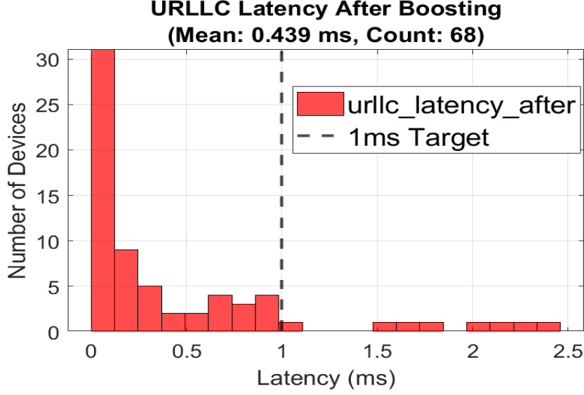
Figure 6: URLLC Latency After Boosting
