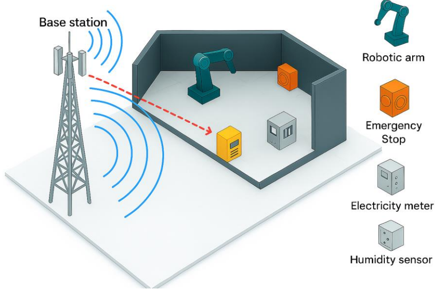
Figure 1: System Architecture
