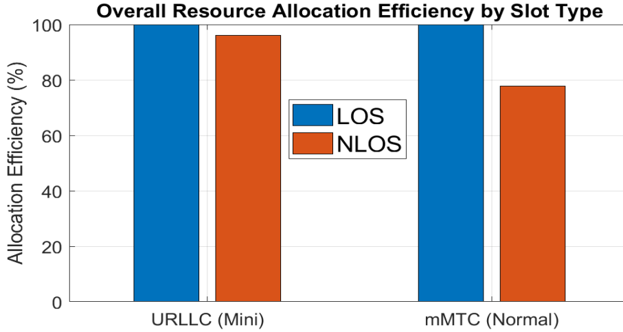
Figure 10: Overall Resource Allocation Efficiency by Slot Type
