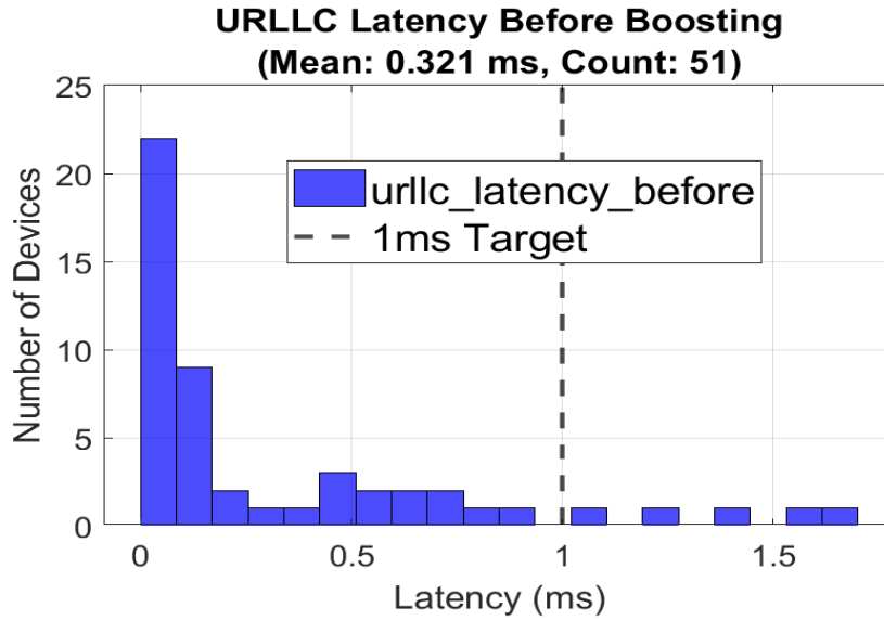
Figure 5: URLLC Latency Before Boosting
