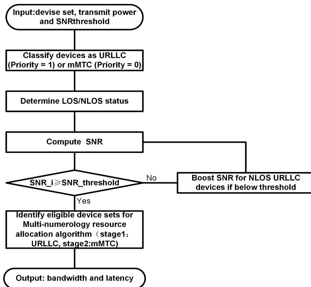
Figure 2: Algorithm Flowchart
